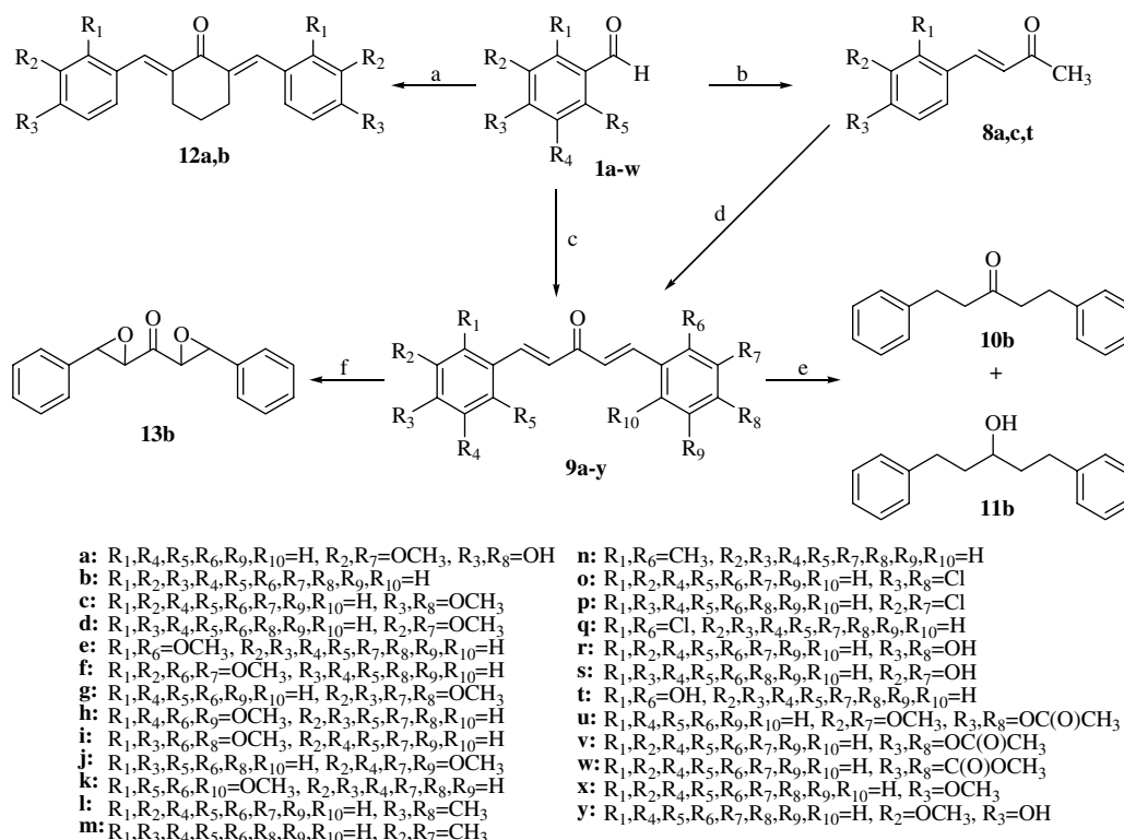
Scheme 2. Reagents: (a) cyclohexanone (0.5 equiv), NaOH, EtOH, H 2 O; (b) CH 3 C(O)CH 3 (1.0 equiv), NaOH, EtOH, H 2 O; (c) CH 3 C(O)CH 3 (0.5 equiv), NaOH, EtOH, H 2 O; (d) PhCHO, NaOH, EtOH, H 2 O; (e) H 2 , Pd/C, EtOAc; (f) Al 2 O 3 -KF, (CH 3 ) 3 COOH, CH 3 CN, ClCH 2 CH 2 Cl.
