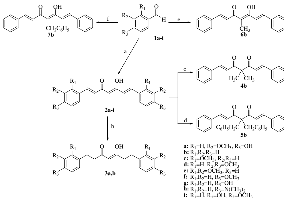
Scheme 1. Reagents: (a) CH_3C(O)CH_2C(O)CH_3 (0.5 equiv), B_2O_3 , B(OC_4H_9)_3 , nBuNH_2 , EtOAc; (b) H_2 , Pd/C, EtOAc; (c) CH_3Br (2.0 equiv), NH_4Cl , NaOH, CH_2Cl_2 ; (d) C_6H_5CH_2Br (2.0 equiv), NH_4Cl , NaOH, CH_2Cl_2 ; (e) CH_3C(O)CH(CH_3)C(O)CH_3 (0.5 equiv), B_2O_3 , B(OC_4H_9)_3 , nBuNH_2 , EtOAc; (f) CH_3C(O)CH(CH_2C_6H_5)C(O)CH_3 (0.5 equiv), B_2O_3 , B(OC_4H_9)_3 , nBuNH_2 , EtOAc.
