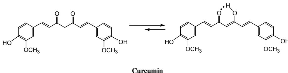
Figure 1. Curcumin exists in solution as an equilibrium mixture of the symmetrical dienone and the keto-enol tautomer stabilized by intramolecular H-bonding.
