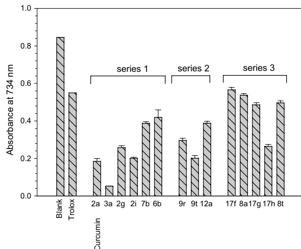
Figure 2. Activities of curcumin and analogues in the TRAP assay. All compounds were tested in triplicate at 10 \mu\text{M} concentrations, with Trolox, 10 \mu\text{M} , as reference standard. All of the remaining analogues were indistinguishable from the blank.
