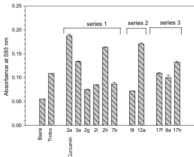
Figure 4. Activities of curcumin and analogues in the FRAP assay. All compounds were tested at 10 \mu M with Trolox, 1 \mu M, as reference standard. All of the remaining analogues were indistinguishable from the blank.
