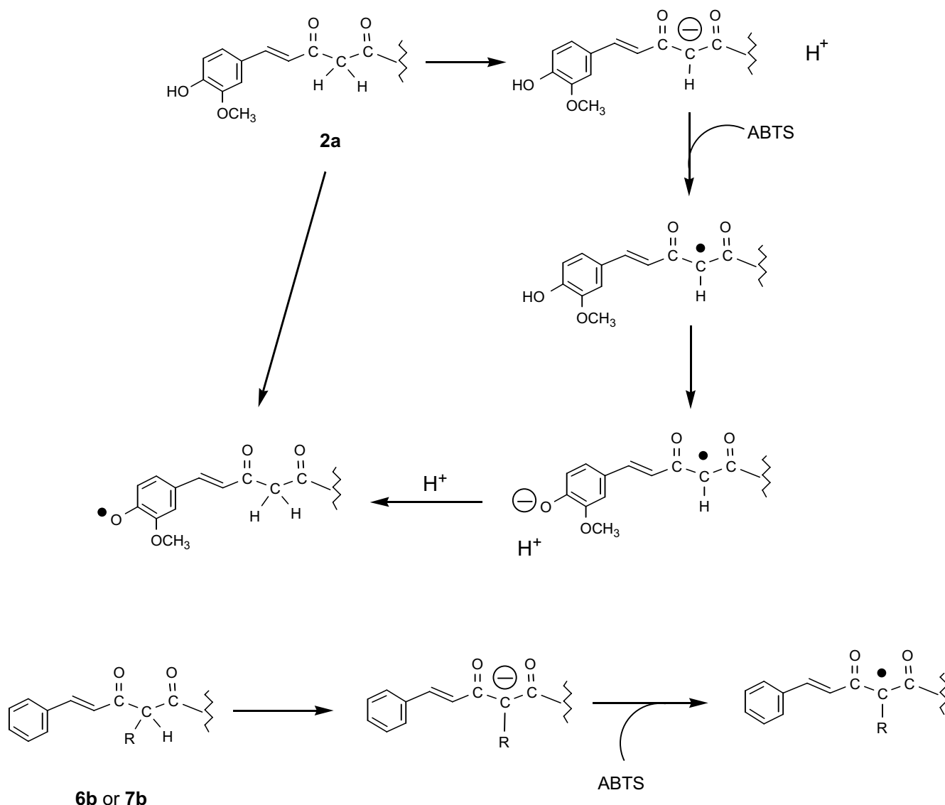
Figure 3. Mechanisms of the radical trapping reactions of curcumin (top) and non-phenolic analogues of curcumin (bottom).
